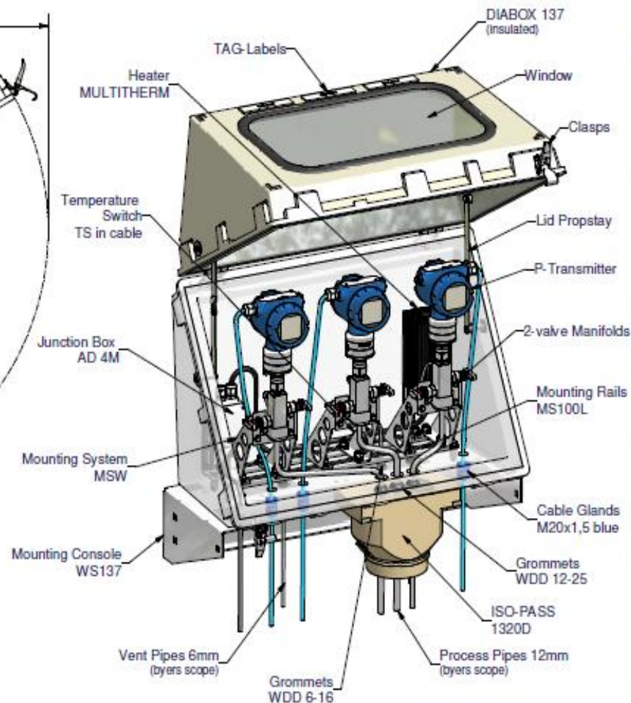
General view
