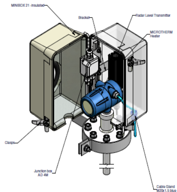
General view
