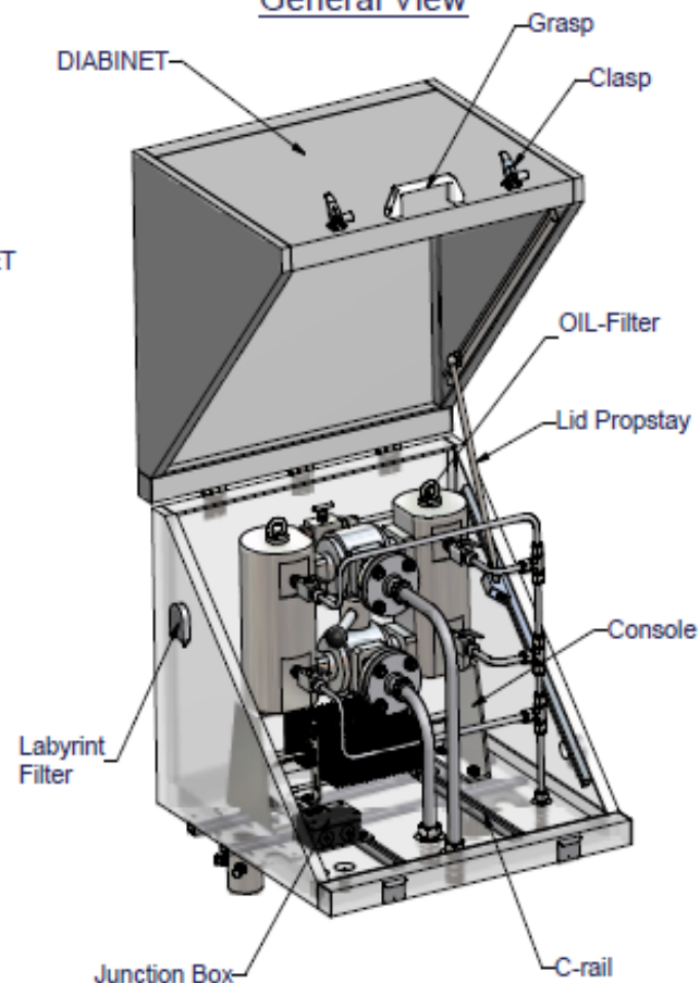
General View
