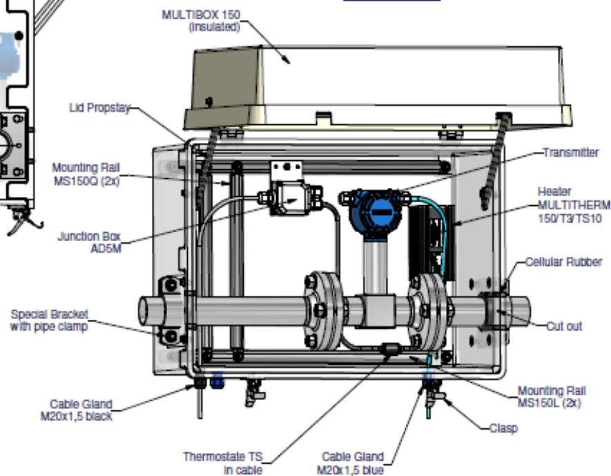
General view
