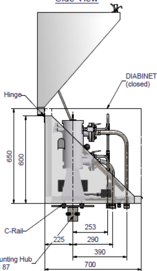
Side View
